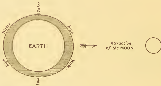
FIG. 112.—Earth and moon (earth's rotation neglected).
